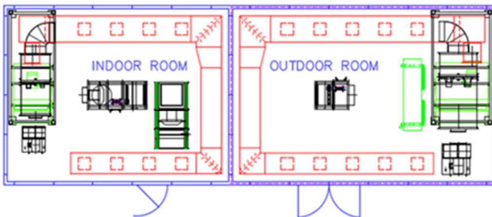
Figure 2.3 Schematic Diagram for the Testing Facility
