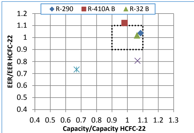
Figure 3.7a CC and EER at 35 C compared to HCFC-22 for Decorative Splits
