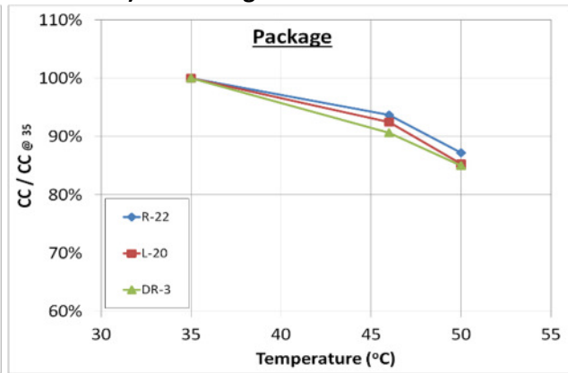
Figure 3.12b CC degradation at high ambient temperatures (percentage compared to 35 C) for Packaged Units
