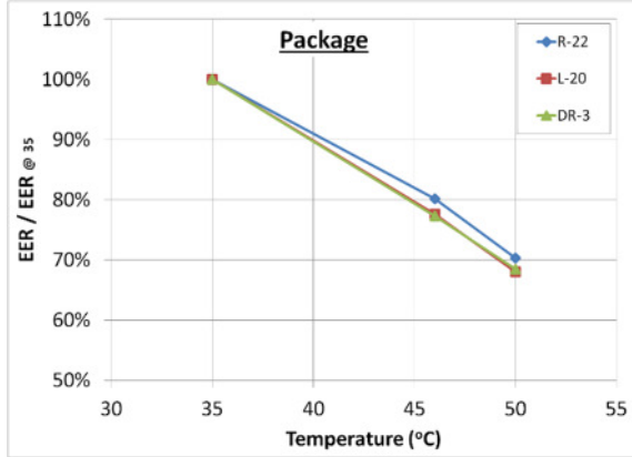
Figure 3.12a EER degradation at high ambient temperatures (percentage compared to 35 C) for Packaged Units
