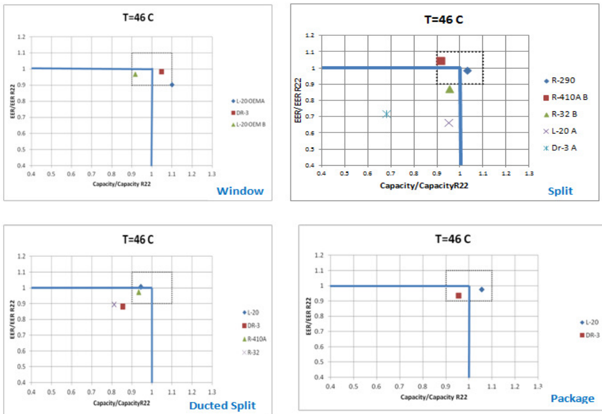
The figure below plots the cooling capacity vs. energy efficiency, represented by EER, compared as a percentage to the baseline unit of each category. A +/- 10% box is drawn; indicating that alternatives that fall within the box are potential suitable candidates.
