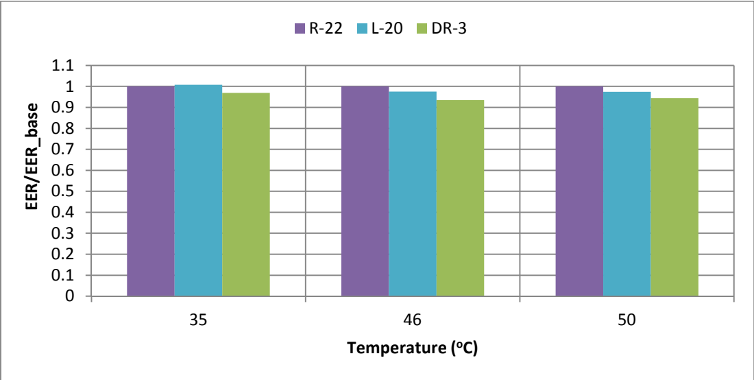
Figure 3.11b EER of Packaged unit Prototypes compared to HCFC-22 base
