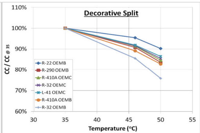
Figure 3.6b CC degradation Decorative Split
