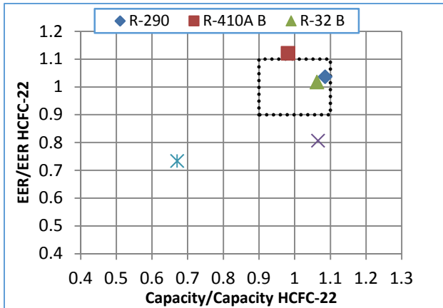
Figure 3.7a CC and EER at 35 C compared to HCFC-22 for Decorative Splits
