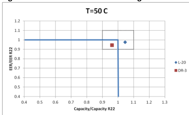
Figure 3.13c EER vs. CC at 50 C –Packaged unit
