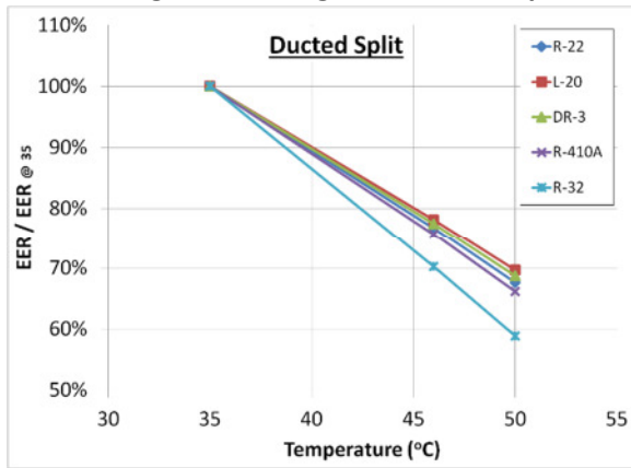
Figure 3.9a EER degradation
