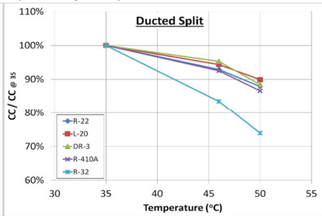
Figure 3.9b Cooling capacity degradation for all refrigerants at high ambient temperatures (percentage compared to 35 °C)
