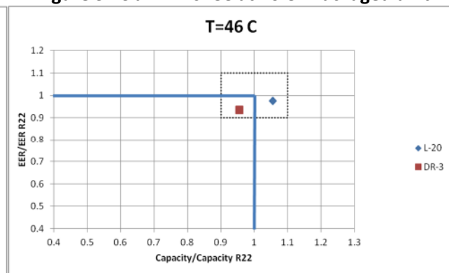
Figure 3.13b EER vs. CC at 46 C –Packaged unit
