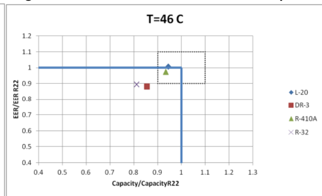
Figure 3.10b EER vs. CC at 50 C for Ducted Splits
